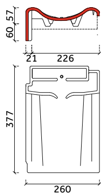
ondergevelpan links
