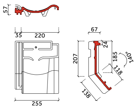
knikpan 140°
