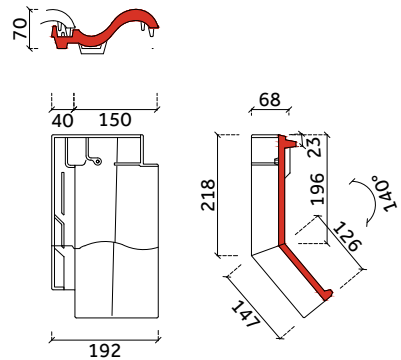
2/3 knikpan 140°
