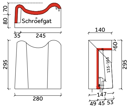
chaperongevelpan links 90°
