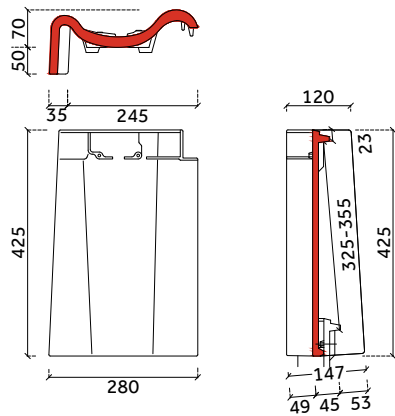
gevelpan links
